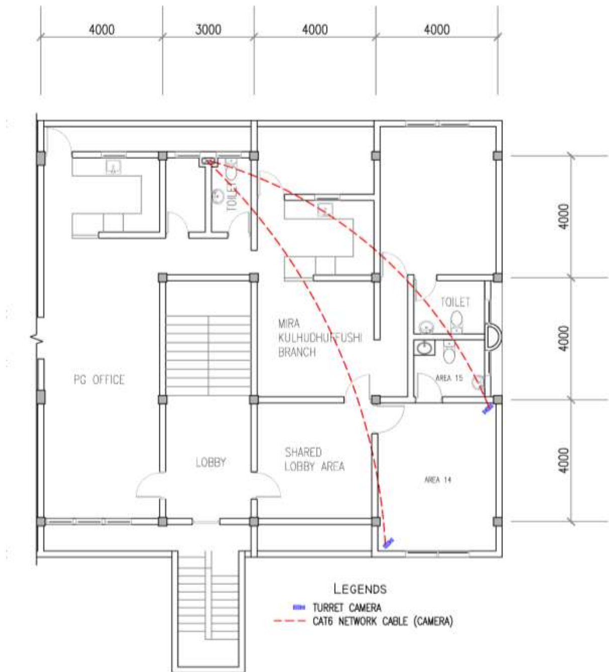
THIRD FLOOR CCTV LAYOUT
